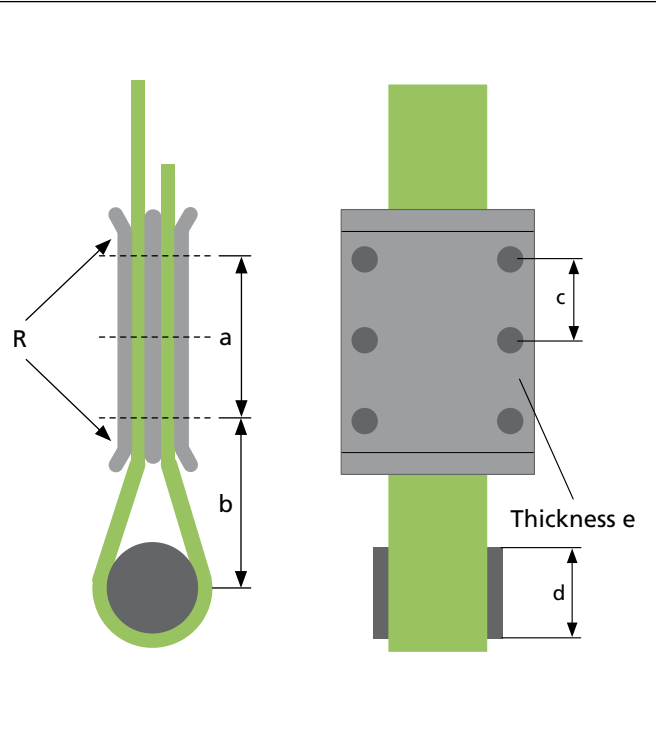
Fastening element Type 1 (pictorial schematic)
