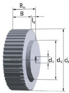
Stock pulleys over z = 44 without flanges
